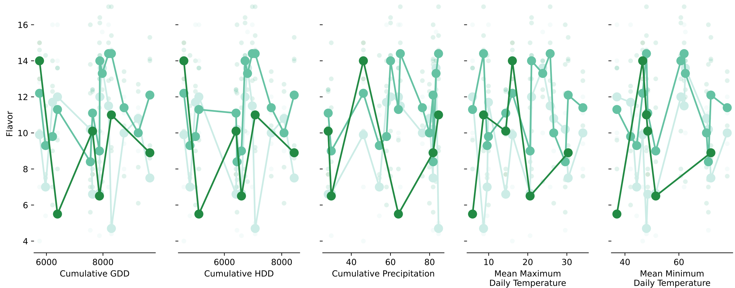
Under Ripe Ripe Over Ripe Climate impacts on Flavor for Marquette, 2019
